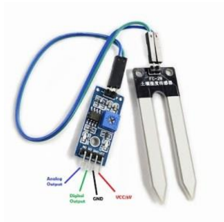
Gambar 2.2 Tampilan fisik sensor soil moisture
